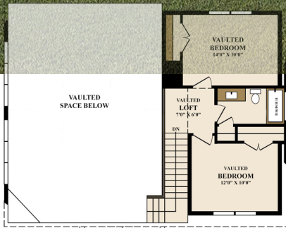
SECOND LEVEL FLOOR PLAN
