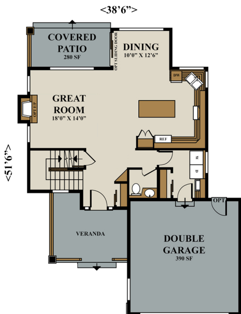
MAIN FLOOR PLAN 856 SQ. FT (79.5 M 2 ) 9'-0" CEILING HEIGHT
