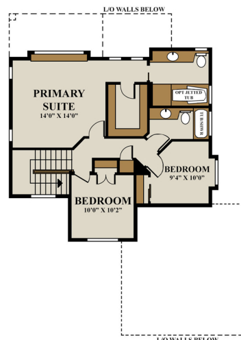
SECOND FLOOR PLAN 841 SQ. FT (78.1 M 2 ) WIDTH - 38' - 6" (11.7M) DEPTH - 51' - 6" (15.7M)
